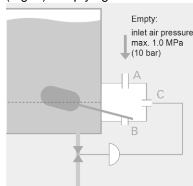
(Fig. 2) Emptying
